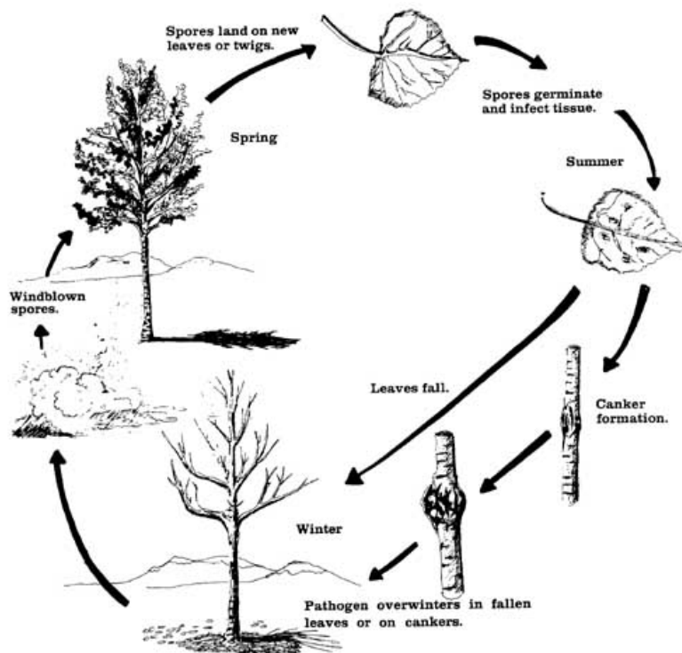
Figure 9: Generalized disease cycle of aspen and poplar leaf spots. Cankers form on trees with shoot blight only.
